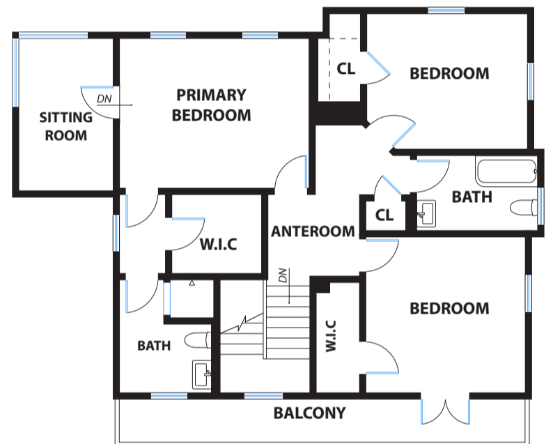
THIRD FLOOR
